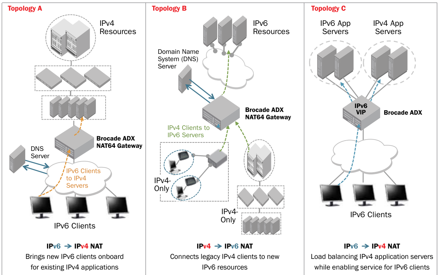
Figure 2. The Brocade ADX NAT64 gateway enables a seamless transition to IPv6.
