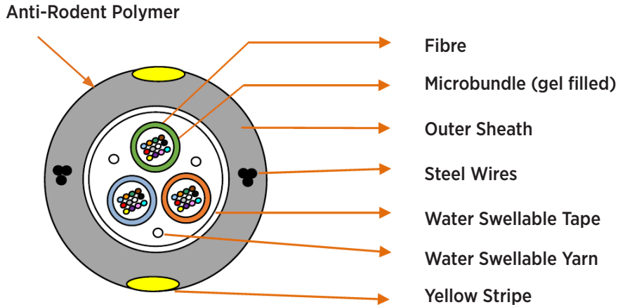
Cross section cable construction of 36-fibre
